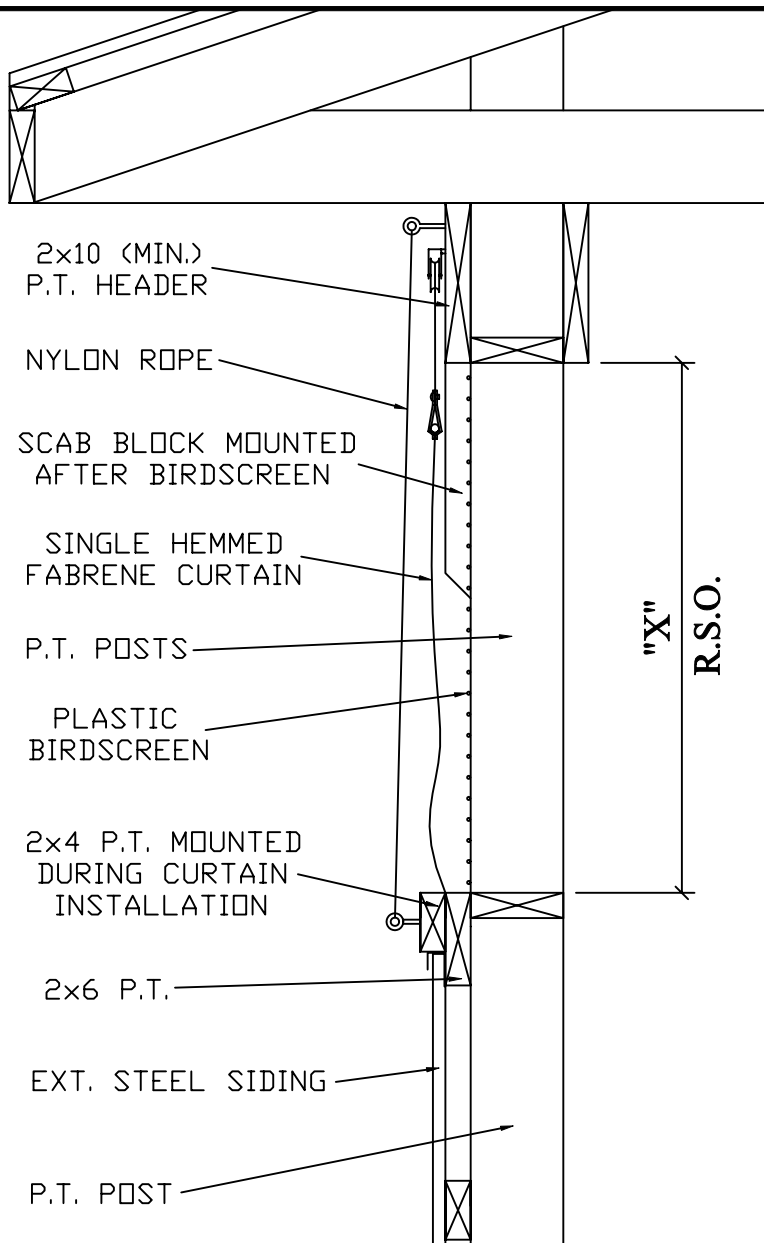
SINGLE HEM CURTAIN WITH BIRDSCREEN AND OUTSIDE ROPE
