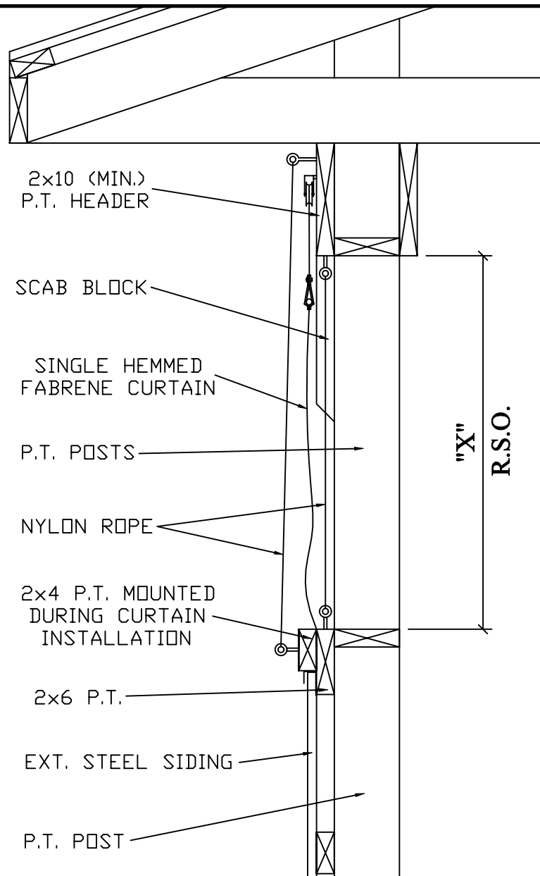
SINGLE HEM CURTAIN WITH DOUBLE ROPE
